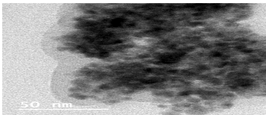
Figure 3: TEM micrograph CdS nanomaterial with of Pr 3+ ion
