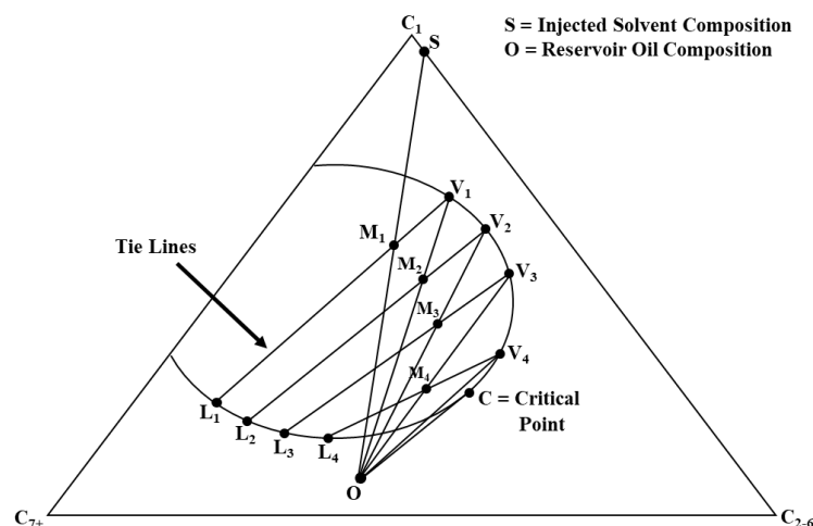
Figure 1: Pseudo Ternary Diagram (Apostolos Kantzas et al. )
