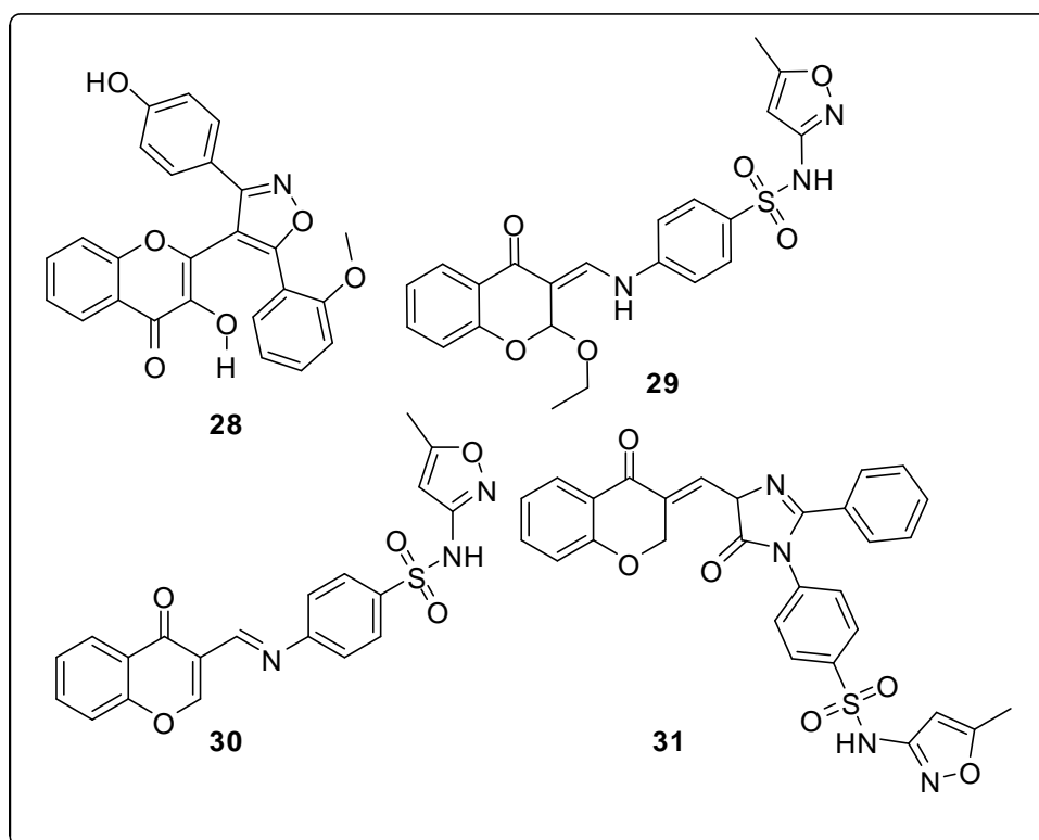
Fig. 12: Flavono-isoxazole derivatives 28-31
