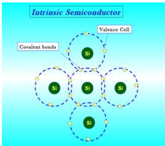
Figure 1: Bond structure
