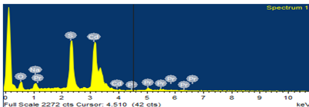
Figure 4: EDAX spectrum of CdS nanomaterial with Pr 3+ ion
