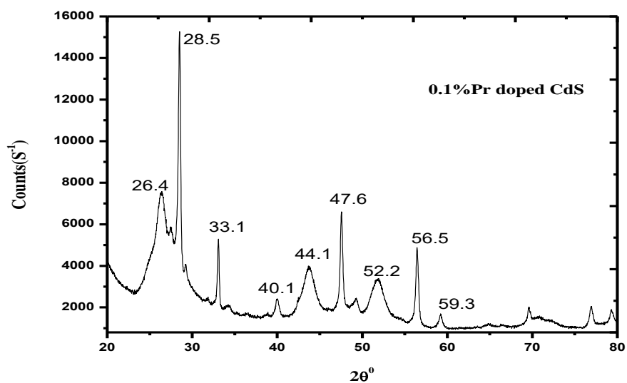
Figure 2: XDR Spectra Pr 3+ doped CdS nanomaterial
