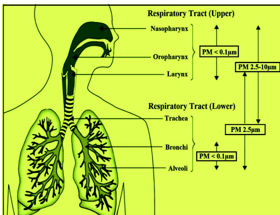
Fig. 1: Size-dependent deposition of particulate matter
