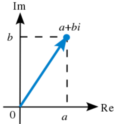
Fig. 1: Argand Diagram
